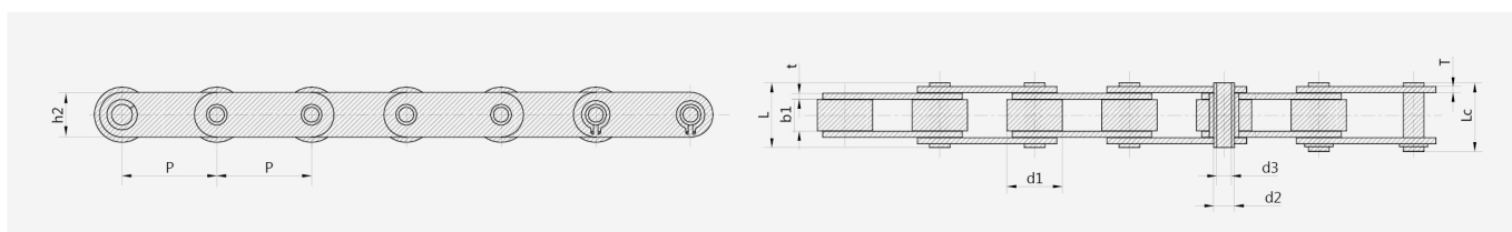
Hollow Pin Chain C Style
